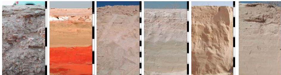
Sandy-skeletal, mixed, hyperthermic Leptic Haplogypsisids Sandy, mixed, hyperthermic Typic Aquisalids Sandy, carbonatic, hyperthermic Typic Petrocalcids Sandy, carbonatic, hyperthermic Typic Torriorthents Mixed, hyperthermic Typic Torripsammments Mixed, carbonatic, hyperthermic Typic Torripsammments
